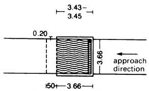
4 Steeplechase water jump: plan
